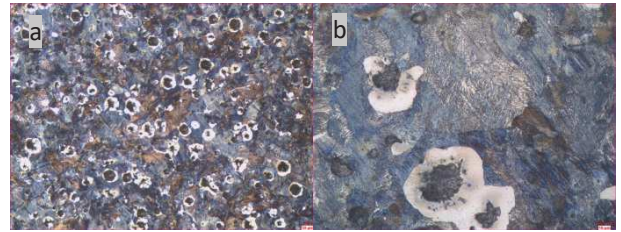
Fig. 2. The microstructure of the cast cam shaft; a) 100x, b) 500x
