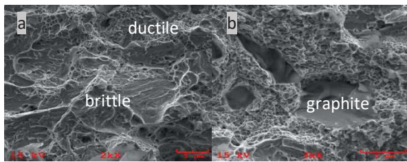
Fig. 7. The images of samples taken from the surface rupture under austempering conditions at 900°C for 60 minutes; a) view of an internal structure exhibiting two different refractive characteristics, b) like brittle fracture of the detail view
