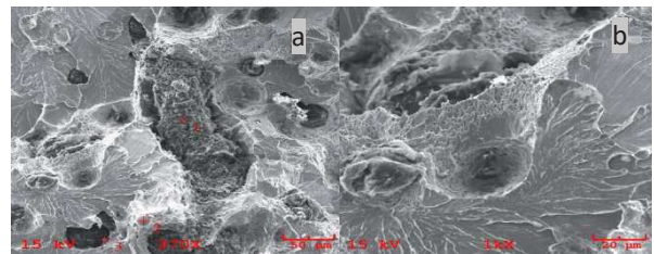
Fig. 6. Review of samples rupture surface under condition of austempering at 800°C for 90 minutes; a) the detail view of the fracture surface with different secondary phases, b) the plastic deformation zone formed along the sides of the secondary phase
