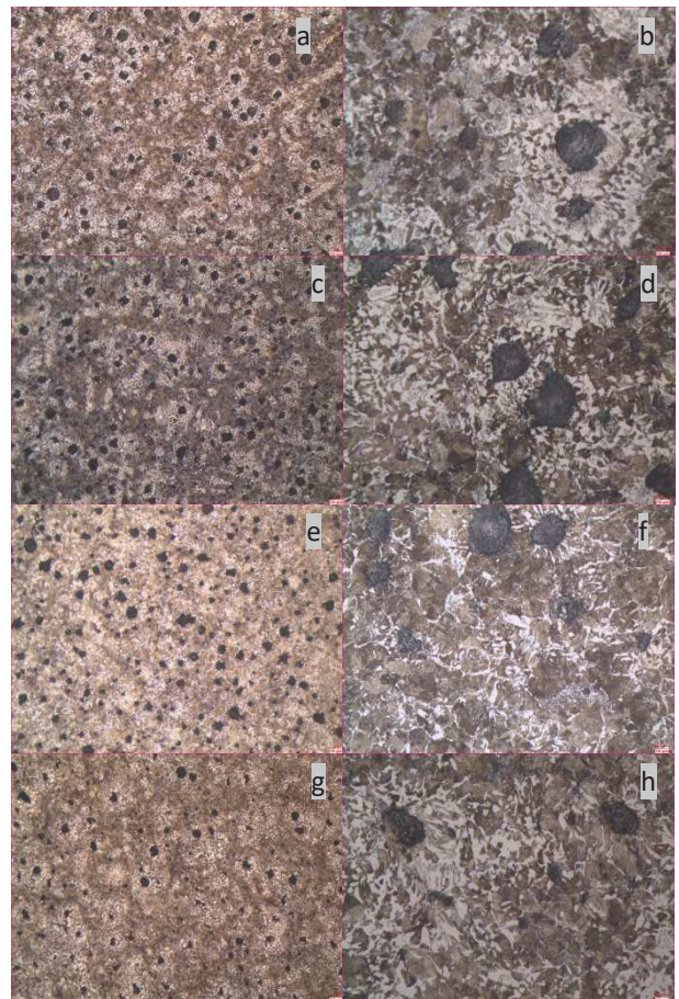
Fig. 3. Microstructures of austempered cam shaft; austenitized at 800°C, 60 min a) 100x, b) 500x; austenitized at 800°C, 90 min c) 100x, d) 500x; austenitized at 900°C, 60 min e) 100x, f) 500x; and austenitized at 900°C, 90 min, g) 100x, h) 500x
