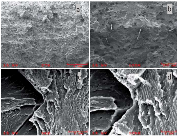
Fig. 4. The SEM images of samples taken from the surface rupture under casting conditions; a) general view, b) a detail from the middle part, c) high magnification matrix details, d) high magnification matrix details
