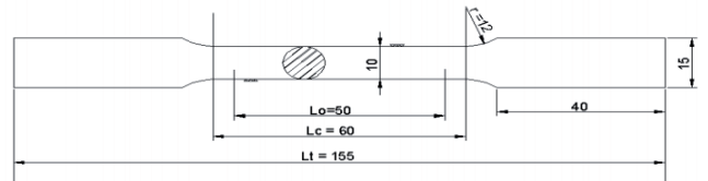
Fig. 1. ASTM A597 standard tensile sample 2D technical drawings
