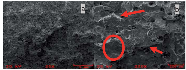
Fig. 5. The images of samples taken from the surface rupture under austempering conditions at 800°C for 60 minutes; a) general view of lower magnifying, b) detail view
