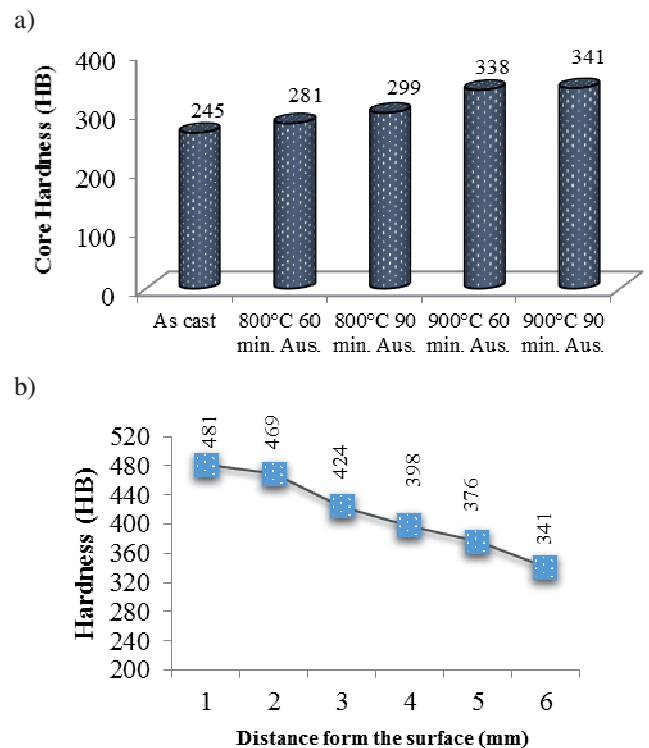
Fig. 9. The results of hardness cam shaft; a) core hardness, b) hardness depth of the surface
