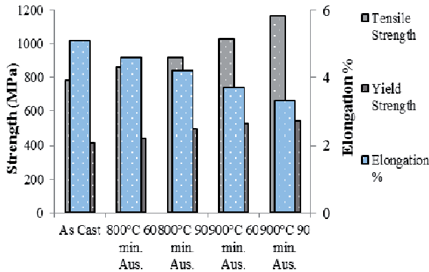
Fig. 10. The results of tensile test
