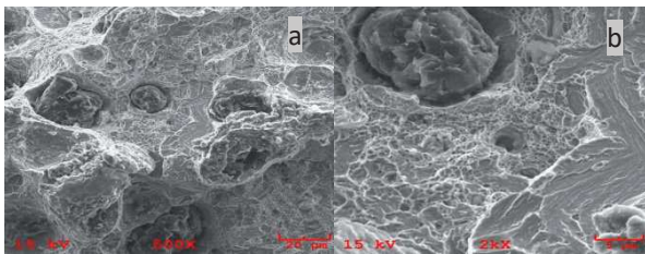
Fig. 8. The images of samples taken from the surface rupture under austempering conditions at 900°C for 90 minutes; a) a detail view through sample, b) a detail from a view; fracture surface contains ductile and brittle fracture characteristics
